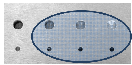
FIGURE 08 & 08A - C-SCAN AND 3D IMAGE
